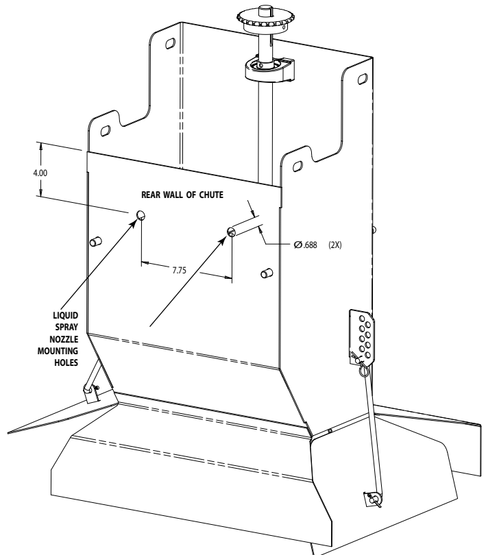
Fig. 5 Liquid Spray Nozzle Location
