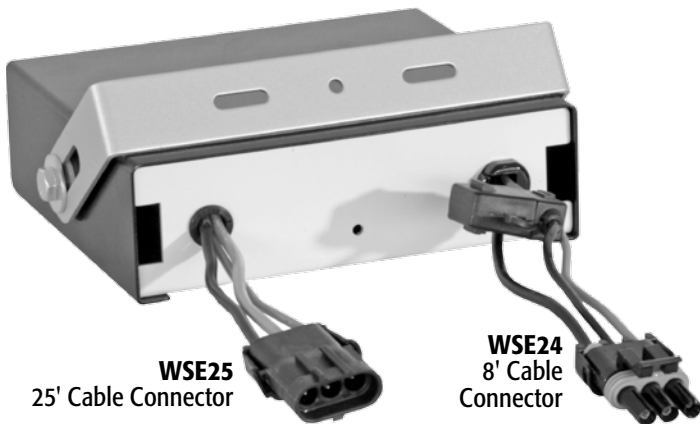
Fig. 3 WSE1 Cab Controller, back view
