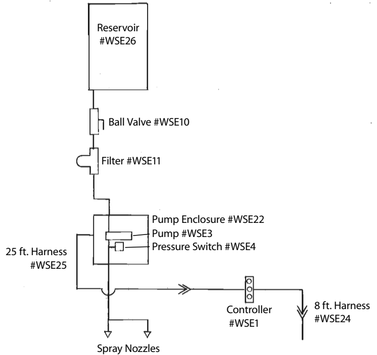
Fig. 4 Plumbing Dia.
